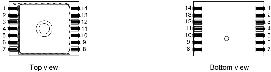
Fig. 2: Pin configuration of MS5536-60CPJU
