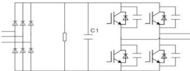
C1: DC-Link
